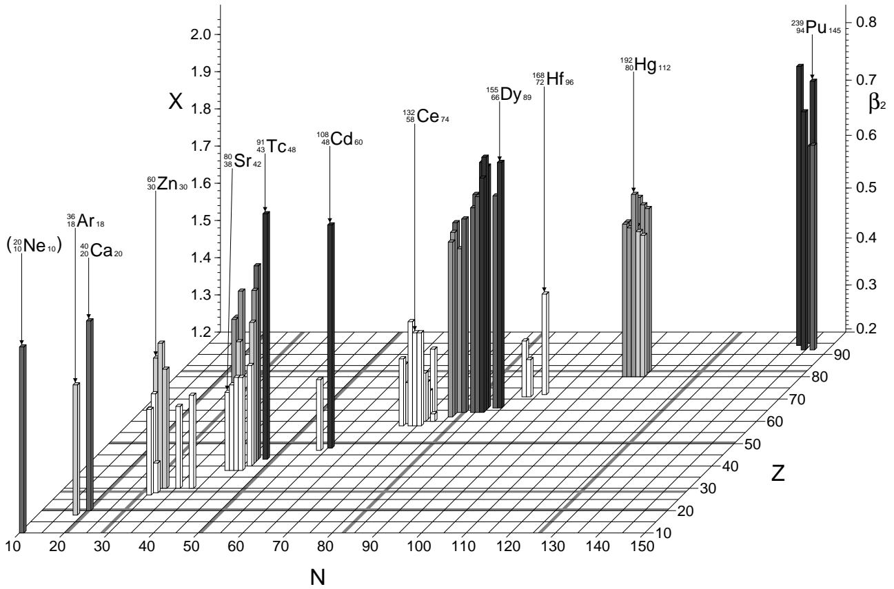
Figure 3. Deformation vs Z vs N
