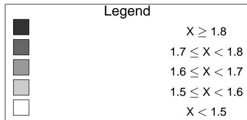
Figure 3. Deformation vs Z vs N
