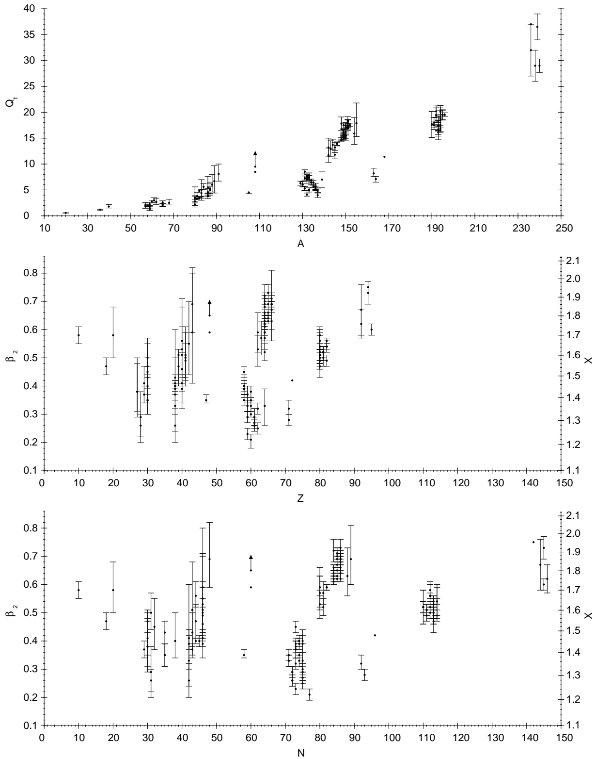
Figure 2. Q_f vs A ; Deformation vs Z and N
